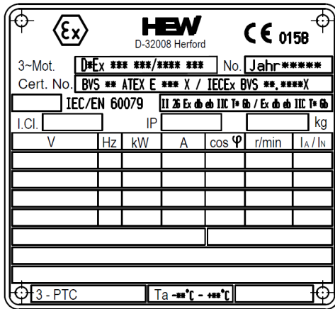
Fig.4: Example of a type plate
